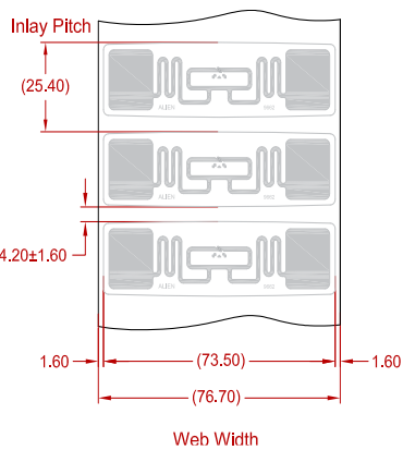
ALN-9662-FWRCA / FWRWA (Clear / White Wet Inlay)
