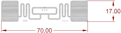
ALN-9662-FRA / FSRA (Dry Unslit / Slit Inlay)
