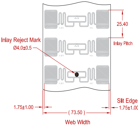
ALN-9662-FSRA (Dry Slit Roll)
