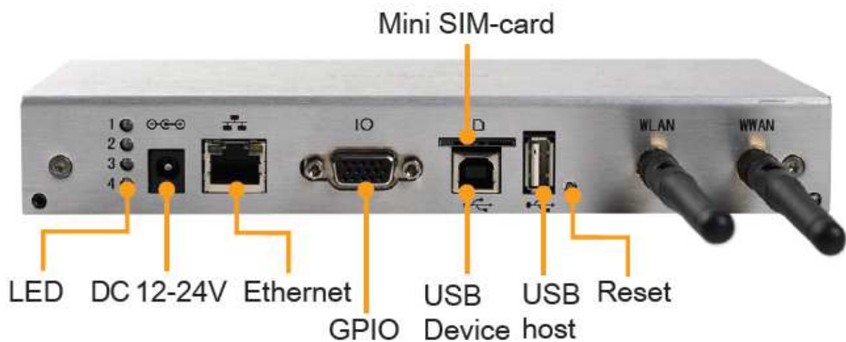
Picture 1 Rear panel of Nordic ID AR62
