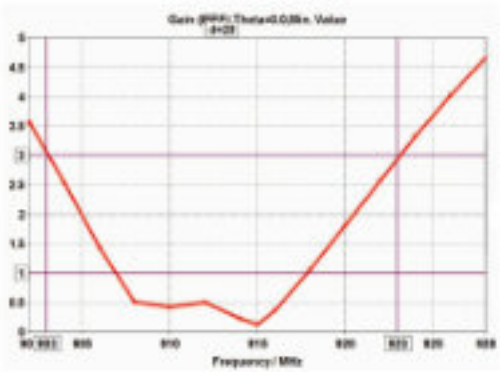
Axial Ratio
