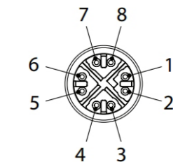
M12 X-Coded female Ethernet Network connector
