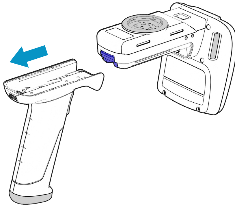
Figure 5: Slide Power Handle off
