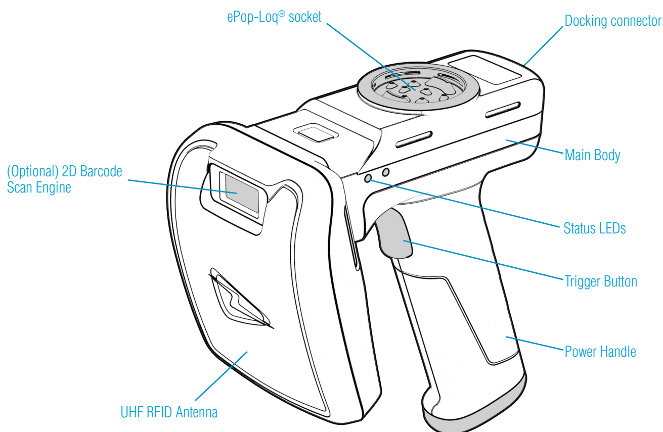
Figure 1: 3138 Reader with UHF RFID Antenna, 2D Barcode Imager and Trigger Handle
